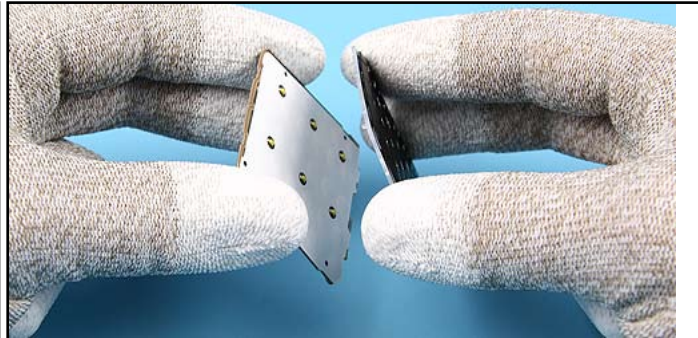
34. Separate the FLIP QWERTY KEYMAT from the FLIP PWB ASSEMBLY
