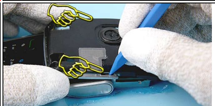
16. The FLIP MODULE is attached to the B-COVER with two snaps.
