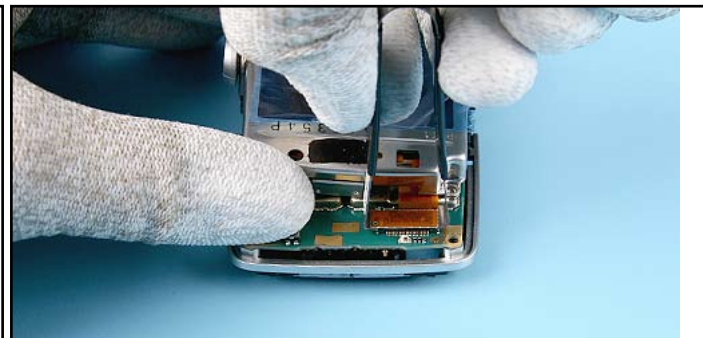
20. Lift the FLIP MODULE a bit and place the flex connector opening tool as shown.
